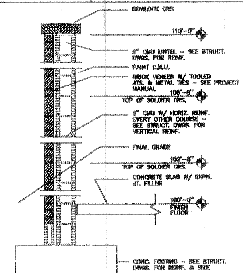
6 SCREEN WALL DETAIL
