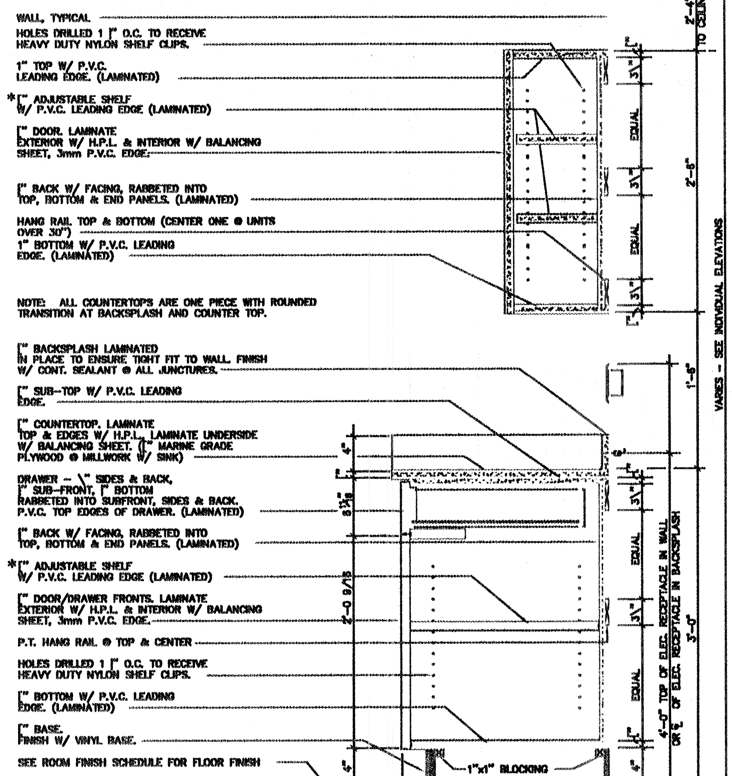
1 TYP. SECTION AT UPPER & LOWER CABINET
